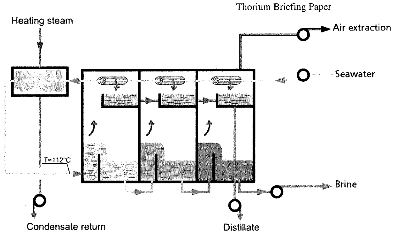
Figure 3: Schematic of Multiple Stage Distiller Source: http://www.sidem-desalination.com/en/Process/MSF/
