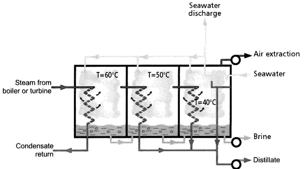
Figure 4: Schematic of Multiple Effect Distiller http://www.sidem-desalination.com/en/Process/MED/
